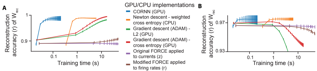
Figure S5: CORNN can be dramatically accelerated with on a standard GPU. The same as in Fig. S2, but with GPU acceleration for CORNN and gradient descent algorithms.
